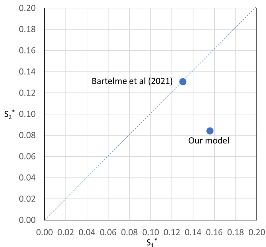
Figure 1: Optimal subsidy rate based on our model and Bartelme et al. (2021)
